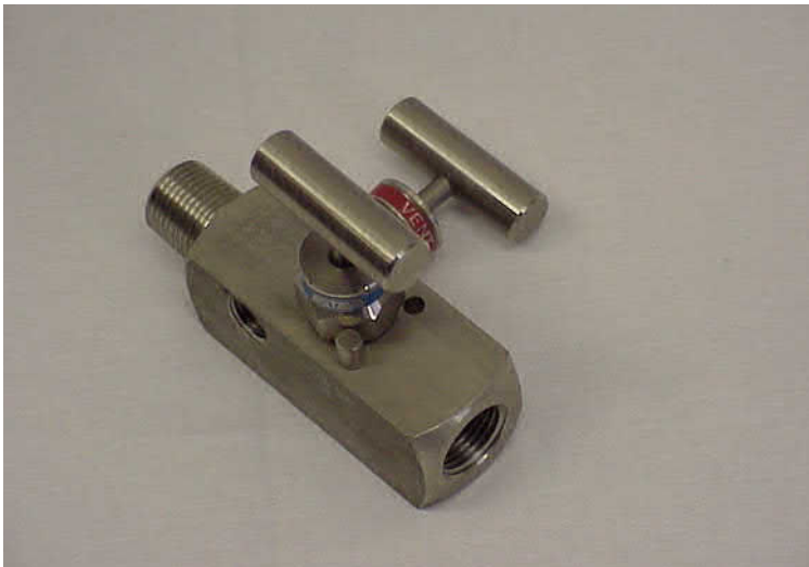
Picture model: 208-06 2-VALVE GAUGE MANIFOLD
